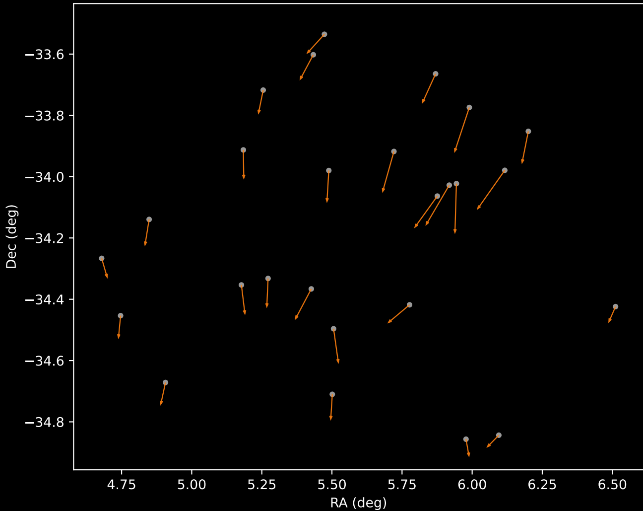
APOGEE DR17 Cluster 2 Proper Motion Vectors (n=26)
