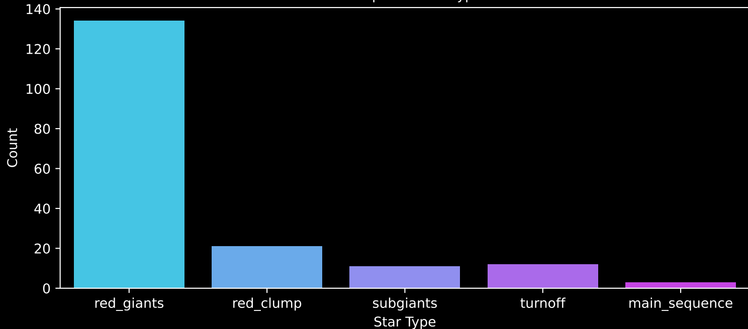
APOGEE DR17 Field: [355-02] Count plot of Star Type
