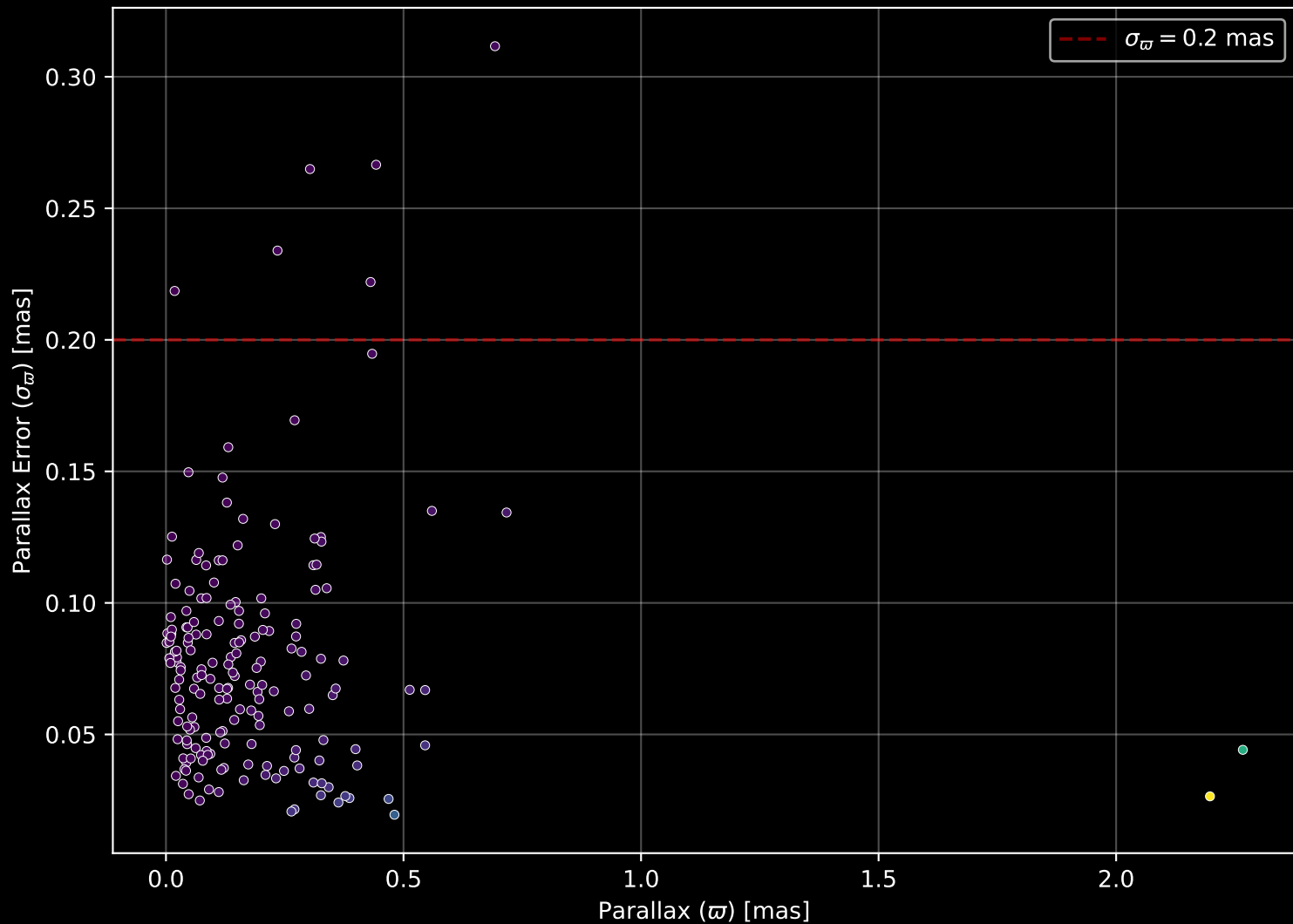
APOGEE DR17 Field: [355-02] Parallax Quality (n= 181)
