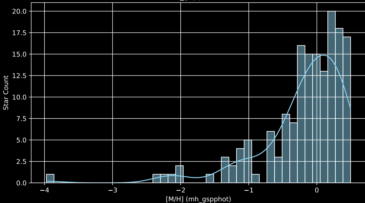
APOGEE DR17 Field: [355-02 [M/H] (mh_gspphot) (n= 160)
