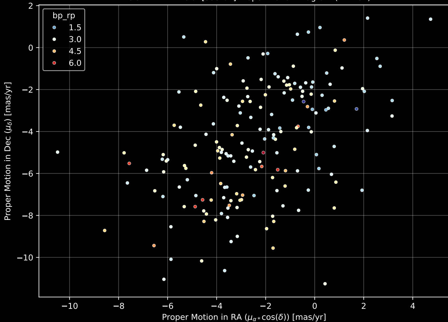
APOGEE DR17 Field: [355-02] Proper Motion Diagram (n= 181)
