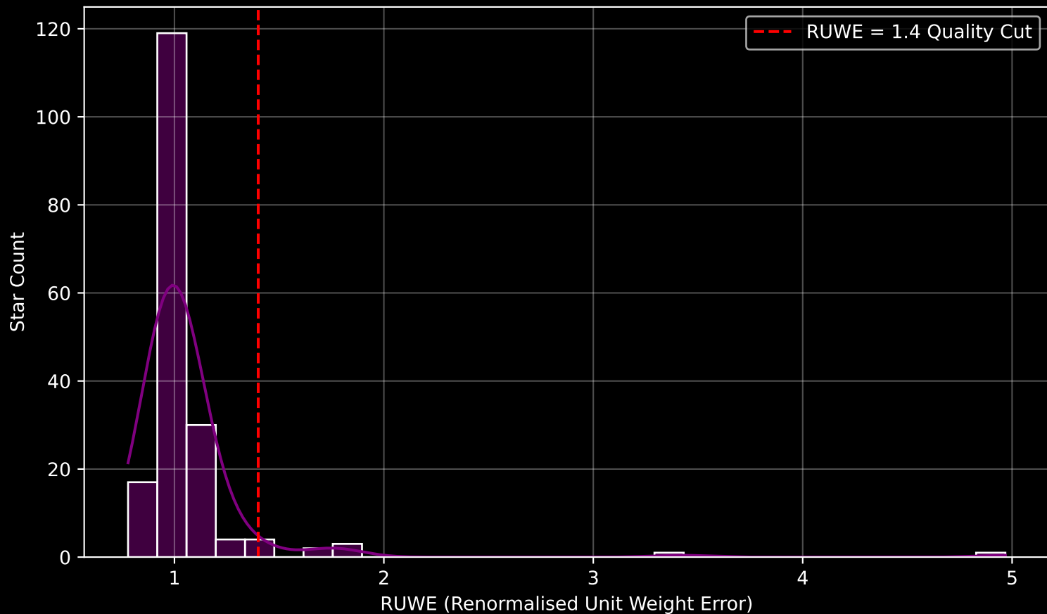
GAPOGEE DR17 Field [355-02] RUWE Distribution (n= 181)
